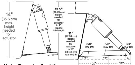
Standard Mount
