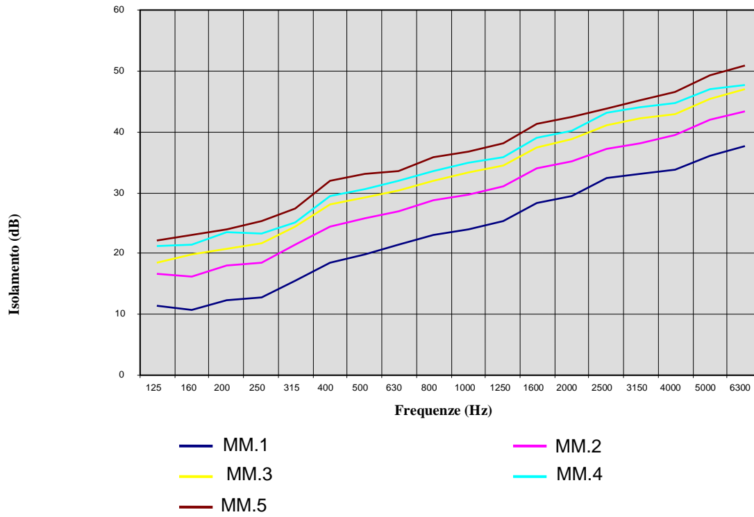
Transmission Loss (DIN 52210)
