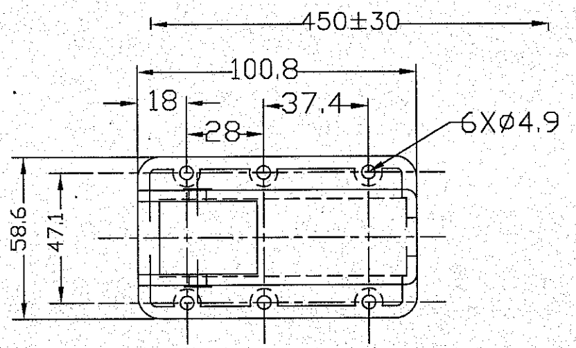
Bracket dimensional diagram
